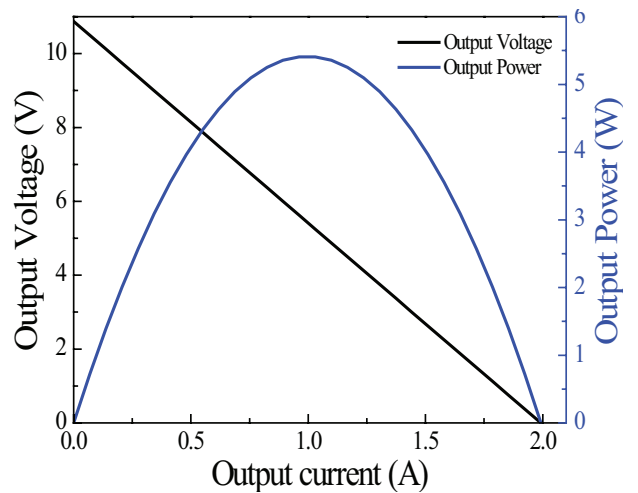
Output Voltage/Power Vs. Output Current (Th=300°C, Tc=30°C)
