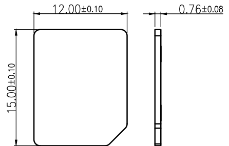
Micro SIM
