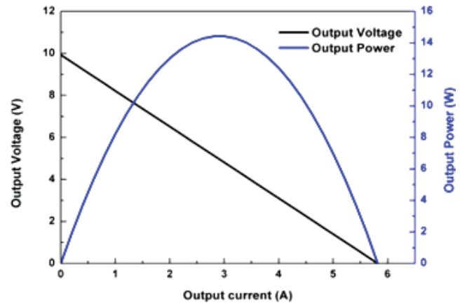
Output Voltage/Power Vs. Output Current (Th=300°C, Tc=30°C)
