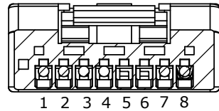
SECTION A-A SCALE 3 : 1 (Back of Connector Housing)
