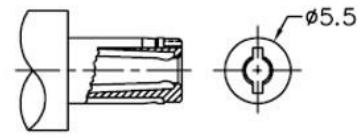
MATING PLUG Jack Insertion Depth: 9.8 mm
